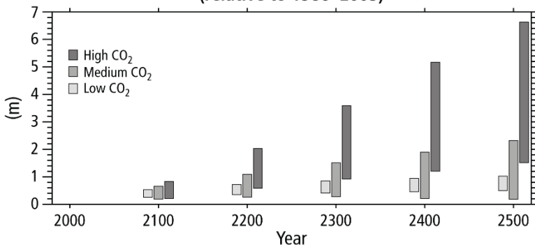
4 (c) Global mean sea level rise (relative to 1986–2005)
