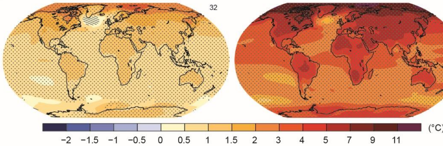
4 (a) RCP 2.6 Change in average surface temperature (1986–2005 to 2081–2100)
